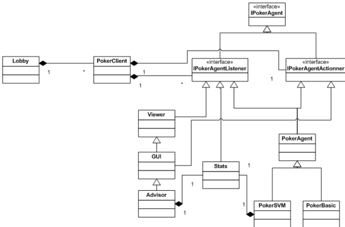
Figure 1 – Architecture côté client
